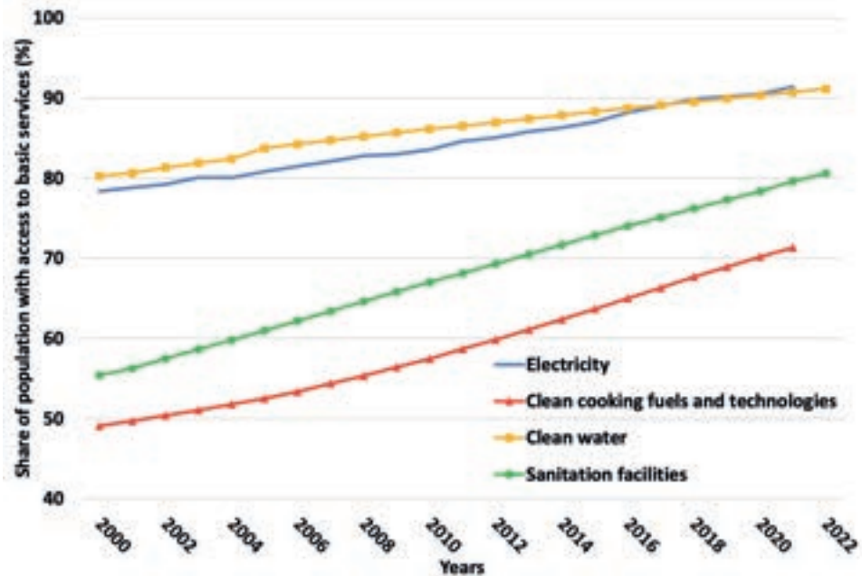
Figure 4 Changes in worldwide access to basic services [Data from (World Bank, 2024b)]
