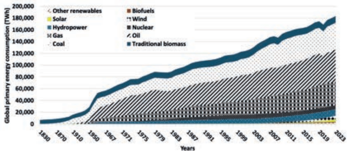
Figure 5 Changes in primary energy consumption in the world by source [Data from (Ritchie et al., 2024)]
